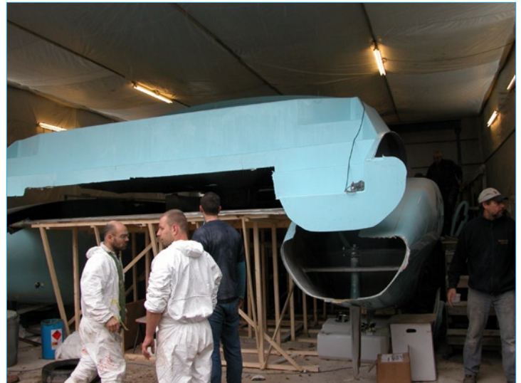
Dazcat 1195 Sueños having bridgedeck introduced to hulls on March 23rd. Fitting together and fit out are taking shape with launching scheduled for April
